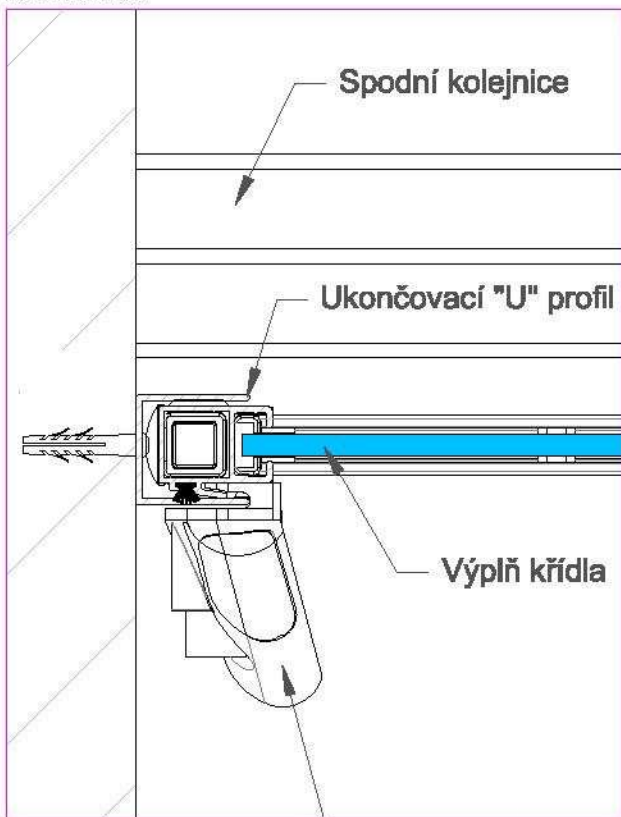
DETAIL C
