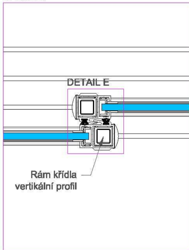
DETAIL D
