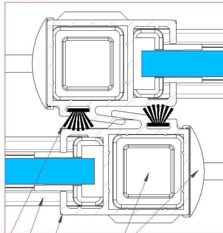
DETAIL E
