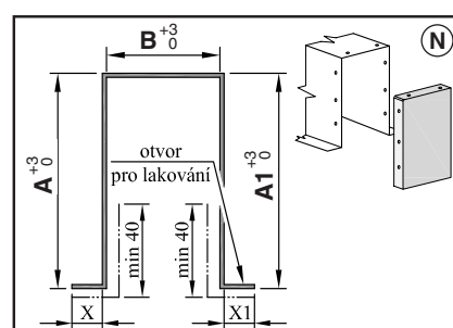
KP 3c L = X + A + B + A1 + X1
