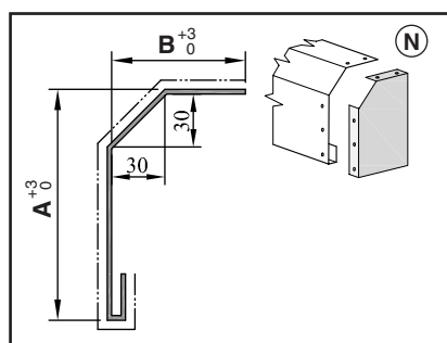
KP 1d L = A + B
