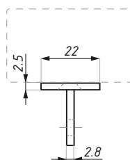
ploché madlo flat handrail
