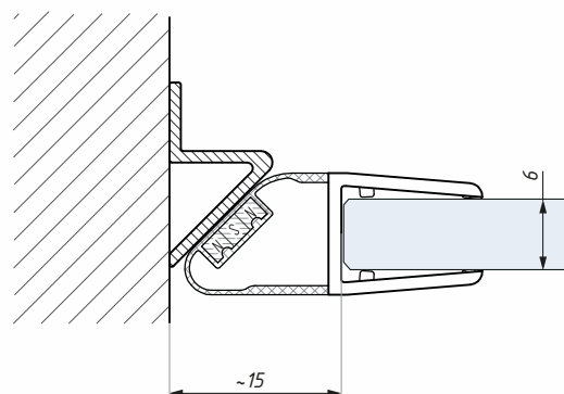
Profil LPMFE 6-8 montáž na sklo 6 mm Profile LPMFE 6-8 for glass 6 mm
