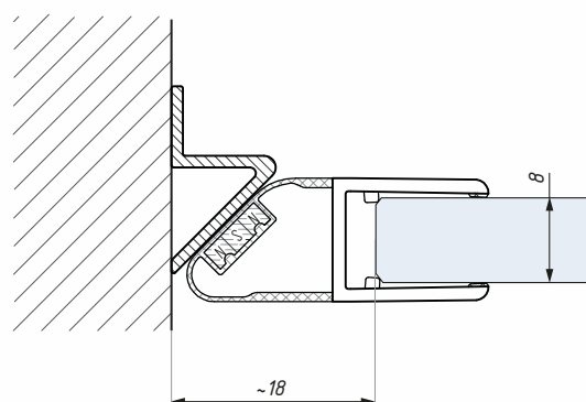
Profil LPMFE 6-8 montáž na sklo 8 mm Profile LPMFE 6-8 for glass 8 mm
